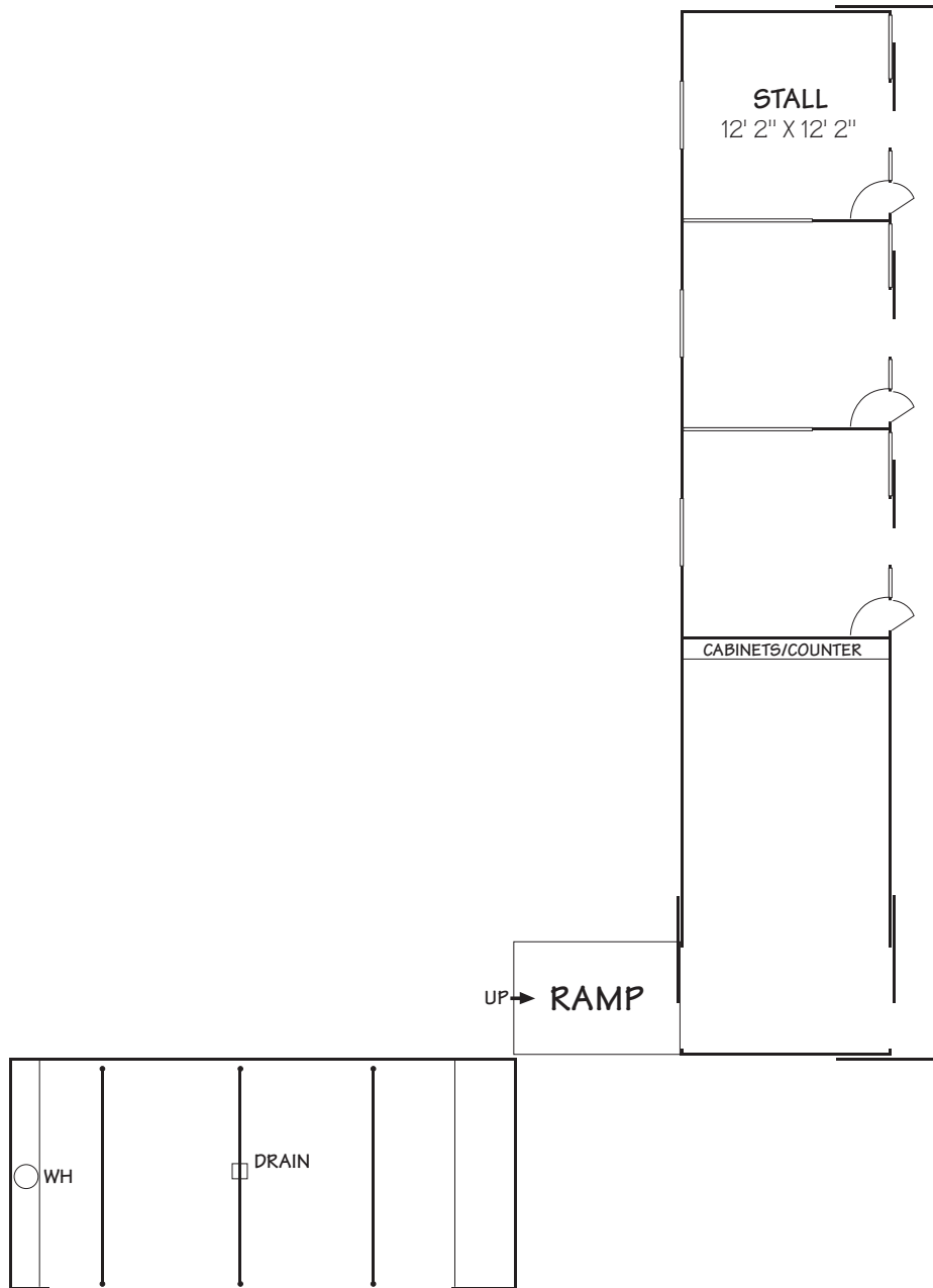
Wash Rack 30'-0" x 13'-8" 409 sq ft
