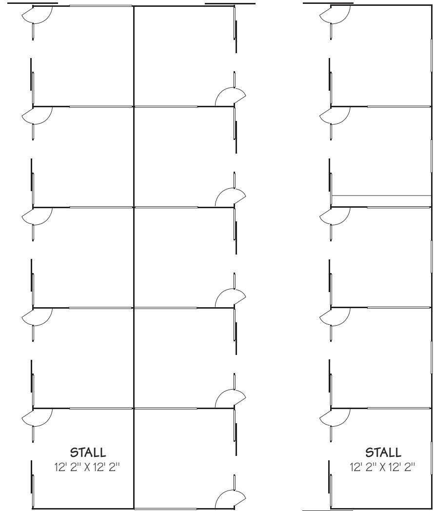
18 Stall Training Barn 73'-2" x 31'-10" 4524 sq ft
