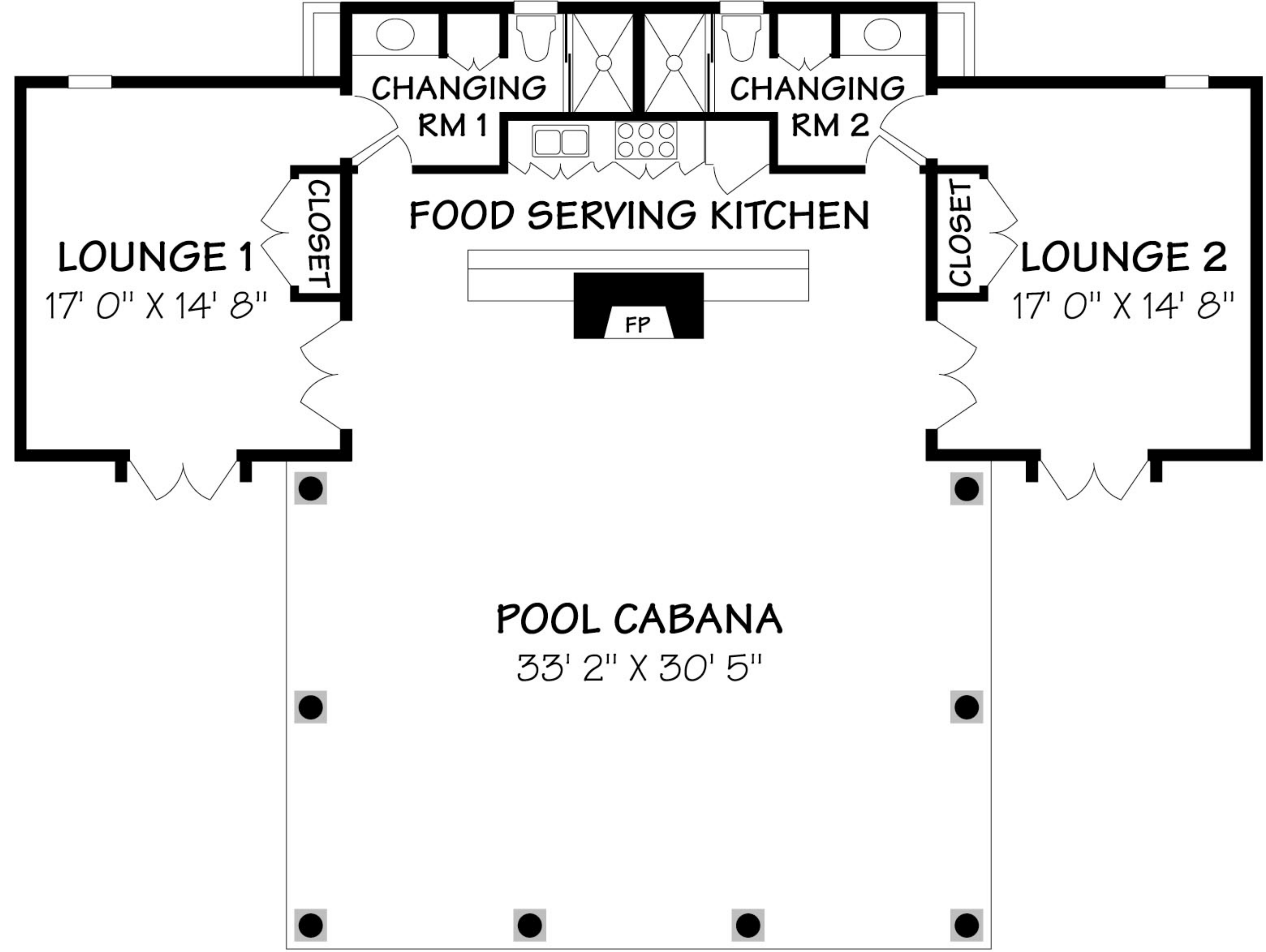
POOL CABANA ±1000 Square Feet
